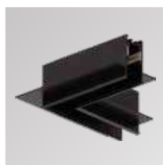
BY41-10101 CRC01 Black Output 48VDC Input 48VAC IP20 Aluminium
