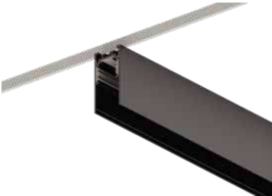
BY41-00211 SR01-1M Black Output 48VDC Input 48VAC IP20 Aluminium BY41-00221 SR01-2M Black Output 48VDC Input 48VAC IP20 Aluminium
