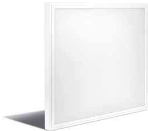
Panelled-SL BP21-06600 BP21-06610 BP21-06630 50W 3000K 5300lm White 220-240V CRI>80 IP20 Iron 50W 4000K 5300lm White 220-240V CRI>80 IP20 Iron 50W 6500K 5300lm White 220-240V CRI>80 IP20 Iron
